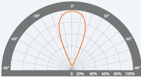
Latitudinal (vertical angle) Polar Radiation Pattern
