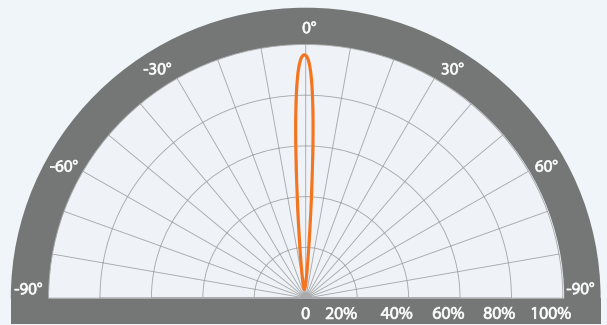
Latitudinal (vertical angle) Polar Radiation Pattern
